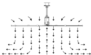
Air flow in an open area
