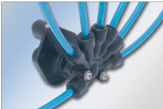
manifold with push-in connections for oil distribution.
