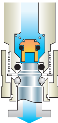
"traditional" quick acting coupler
