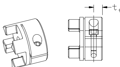
Double Split Clamp Style Hub
