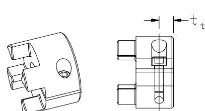
Single Slip Clamp Style Hub
