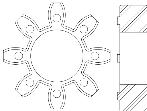
Standard Spider Design
