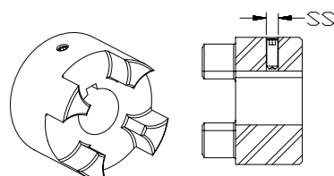
Set Screw Style Hub
