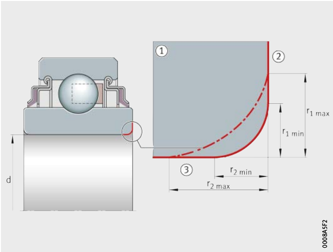
Figure 9 Symmetrical ring cross-section with identical chamfer dimensions on both rings
