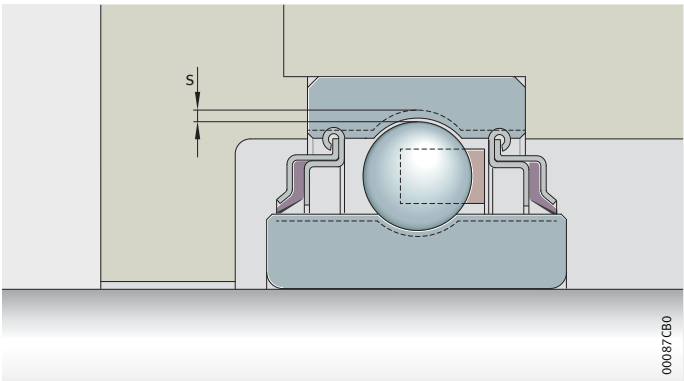
Figure 2 Operating clearance
