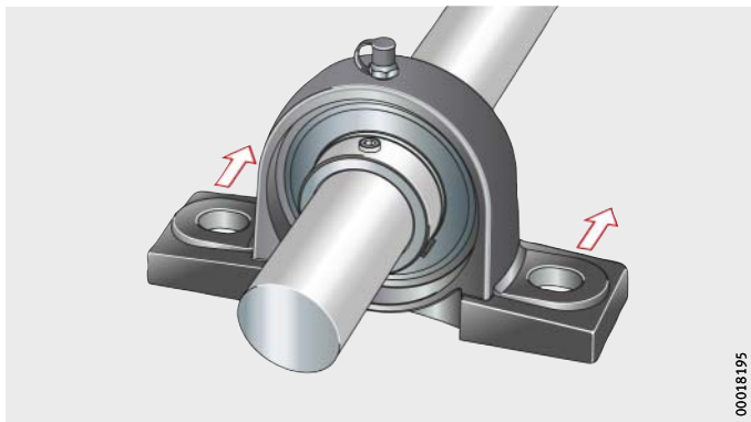
Figure 8 Sliding the unit onto the shaft
