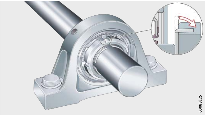
Figure 7 Securing of precision locknut
