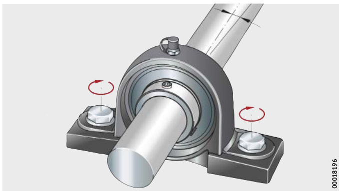
Figure 9 Screw mounting the housing finger tight
