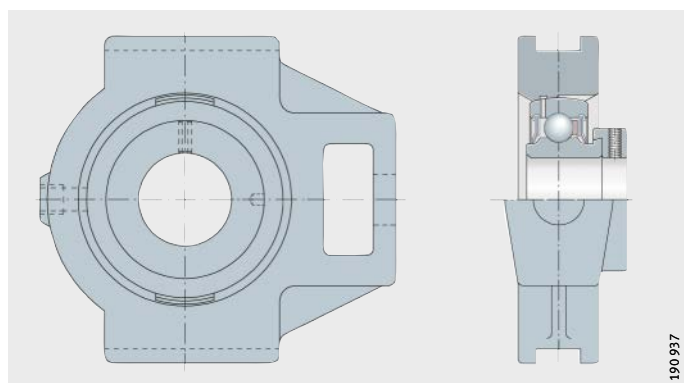
Figure 3 Take-up housing unit, sheet steel housing
