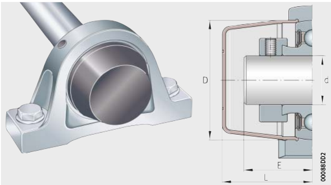
Figure 2 Housing unit with bearing end cap
