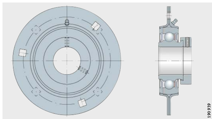
Figure 2 Flanged housing unit, sheet steel housing
