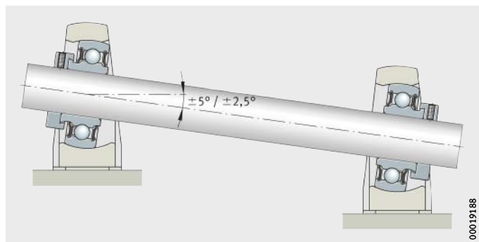
Figure 6 Compensation of static shaft misalignment
