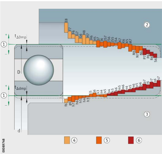
Figure 1 Shaft and housing fits for rolling bearings
