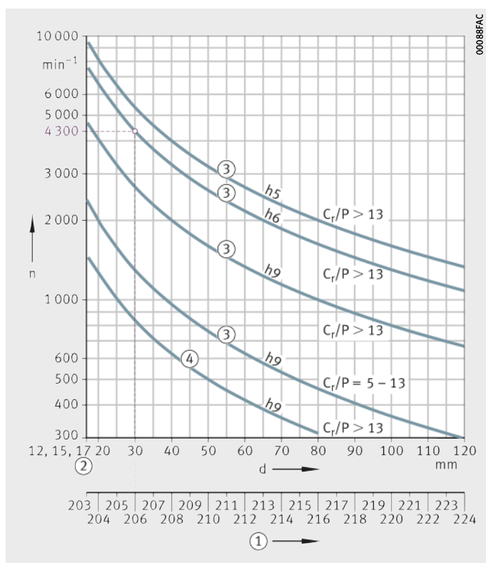
Figure 2 Permissible speeds for radial insert ball bearings
