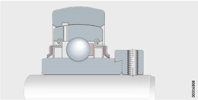
Figure 1 Location by means of eccentric locking collar
