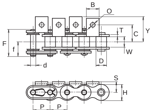
Attachment SA1
