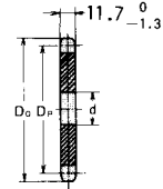
Flat plain (A type)
