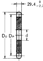
Flat plain (A type)
