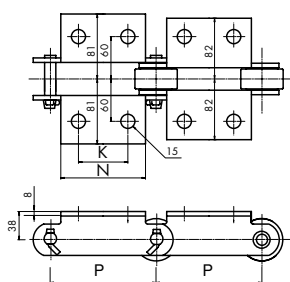
Attachment K2
