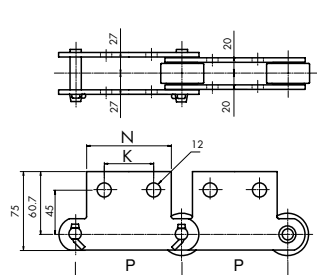
Attachment SK2
