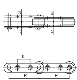
Attachment GK2
