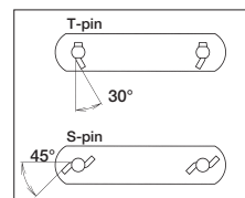
T-pin or S-pin installation method
