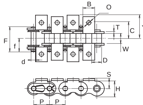
Attachment K1
