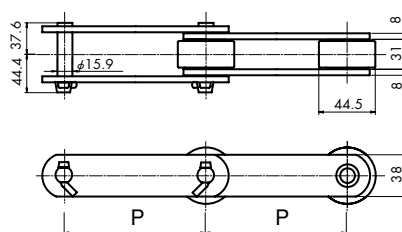
UR-roller
