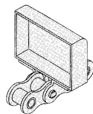
Installation of a bucket with Attachment K1
