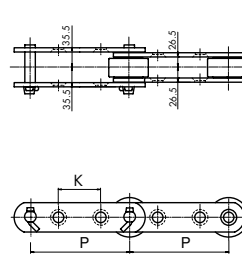
Attachment GK2
