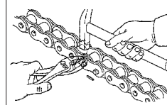
Spring pin installation method for HI-PWR-S series
