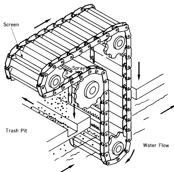
Down Spray Type Travelling Screen
