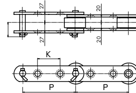
Attachment GK2
