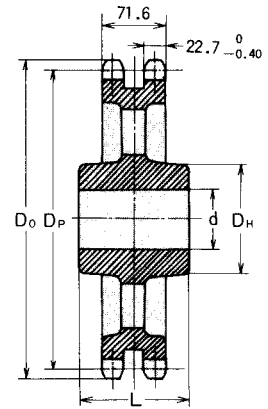
Double sprocket with hub on one side (Double C type)
