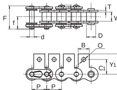
Attachment SK1
