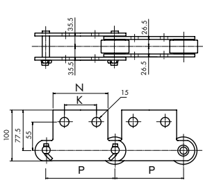
Attachment SK2
