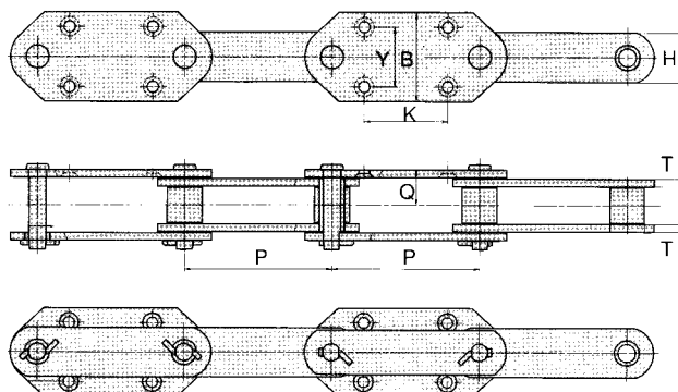
Connecting link (DK100Z or larger)
