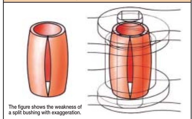
Curled bushing of a standard roller chain
