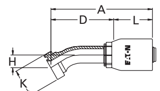
Cat Flange 30° Elbow
