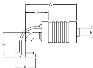
90° Elbow Split Flange FC5053 Code 62
