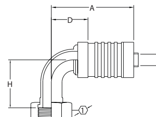
ORS Swivel 90° Elbow (long) FJ9717
