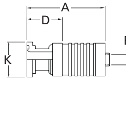
Straight Split Flange FC5050 Code 61 FC5049 Code 62
