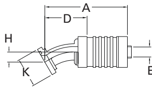
30° Elbow Split Flange FC5612 Code 61 FC5387 Code 62
