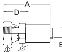
SAE 37° (JIC) Swivel FC9515/FJ9760 FJ9567
