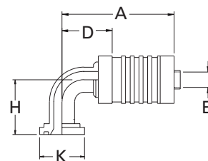
90° Elbow Split Flange FC5329 Code 62
