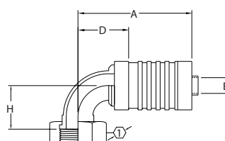
ORS Swivel 90° Elbow (short) FJ9614
