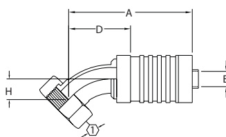
ORS Swivel 45° Elbow FJ9611
