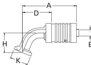
67 1/2° Elbow Split Flange FC5371 Code 62
