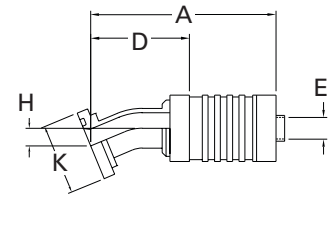
22 1/2° Elbow Split Flange FC5507 Code 61
