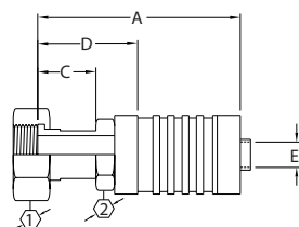
ORS Swivel Straight FJ9608
