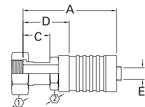
ORS Swivel Straight
