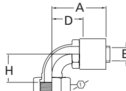
ORS Swivel 90° elbow (short) FJ9612/FJ9898
