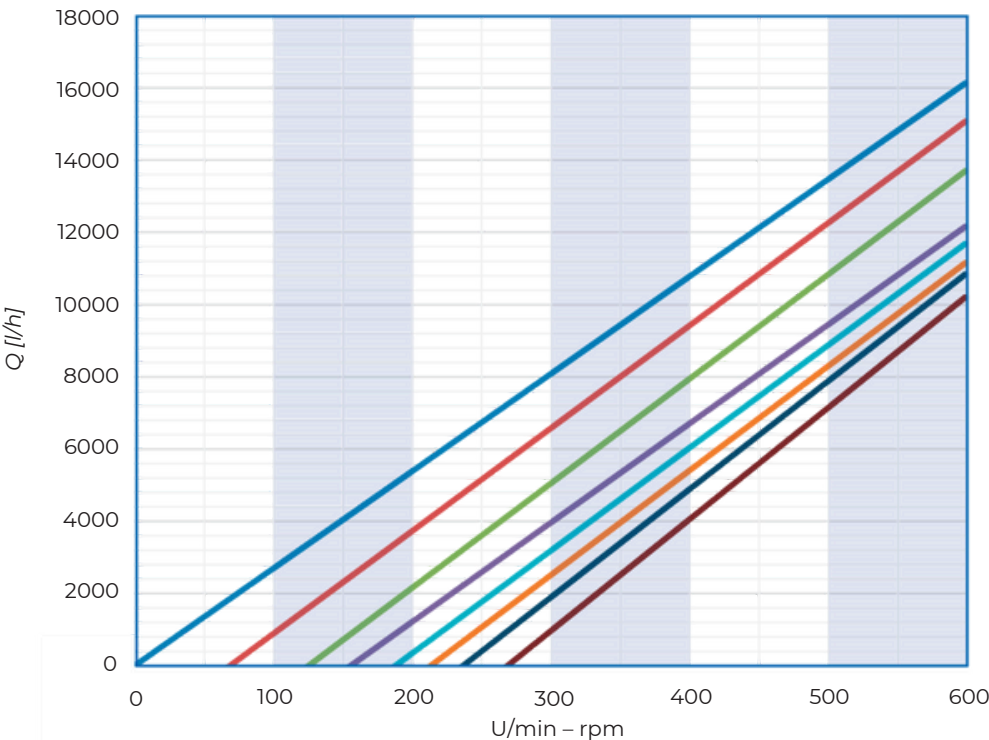
Performance curve depending on the type of medium and the application parameters.
