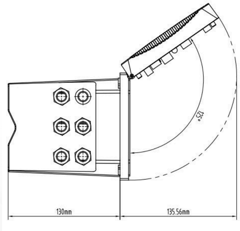
Figure 5 Panel Installation
